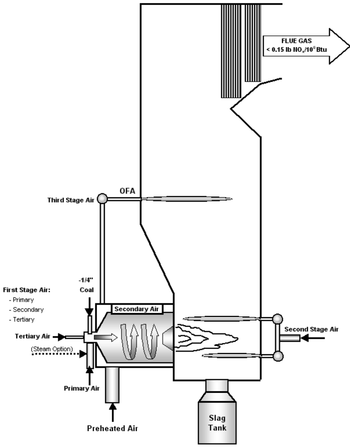
Figure 3. Stage3Cyclone combustion technique.
