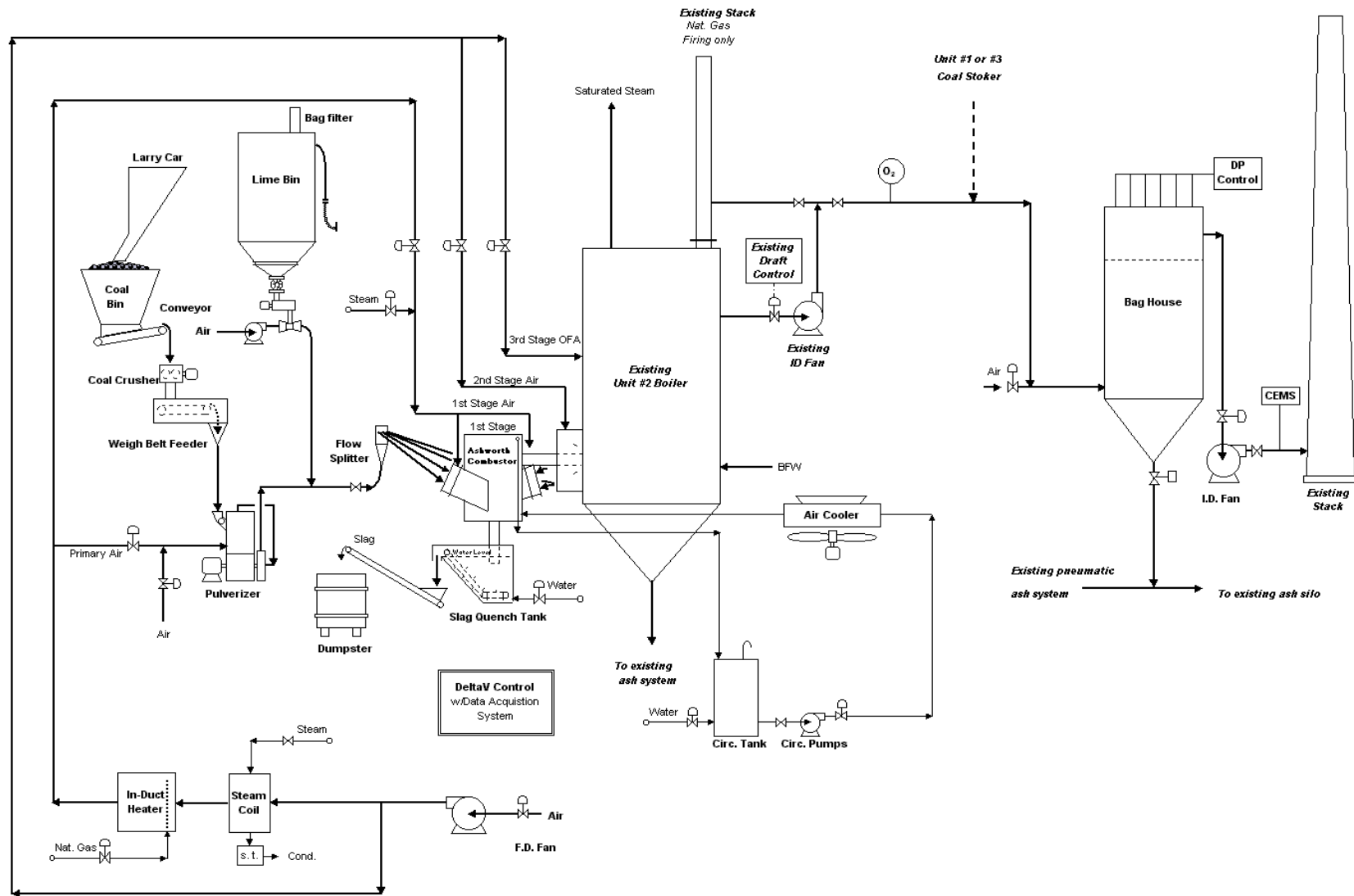
Figure 3. Simplified process flow diagram of Ashworth Combustor retrofit to Lincoln Unit #2.
