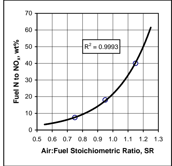
Figure 1b. Fuel N to NO x Conversion
