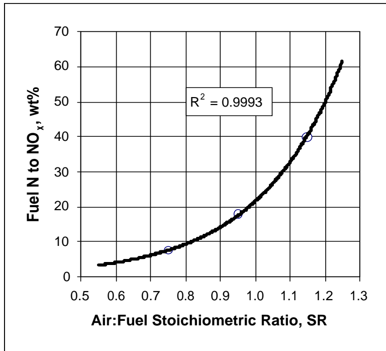
Figure 8. Gasifier SR versus Coal N to NO results.
