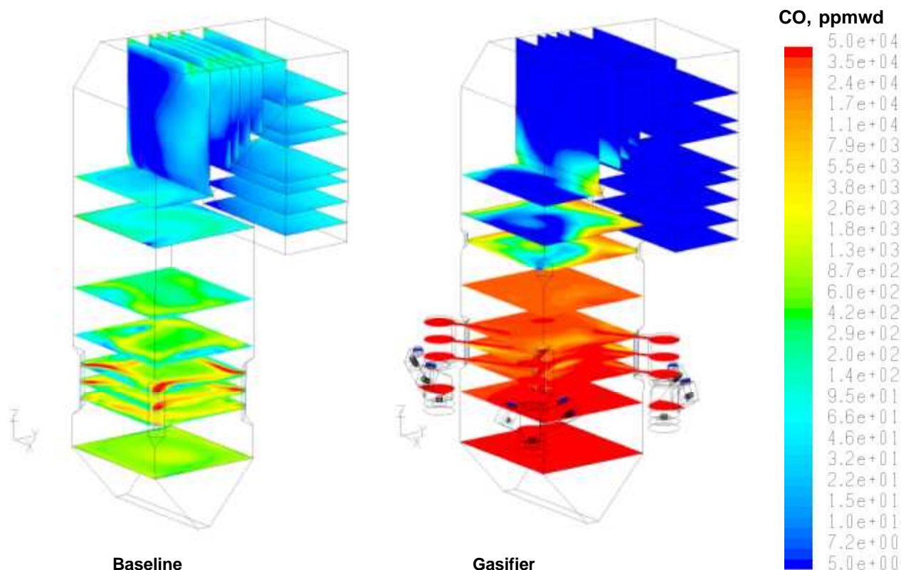
Figure 6. CO distribution comparison.
