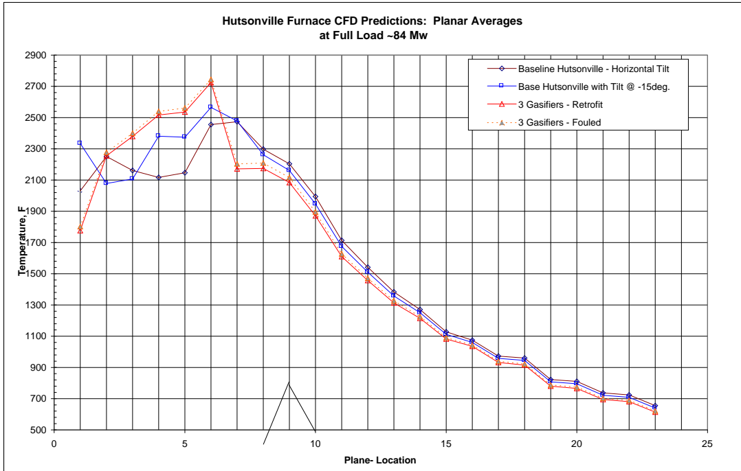
Figure 2. Temperature distribution comparison.
