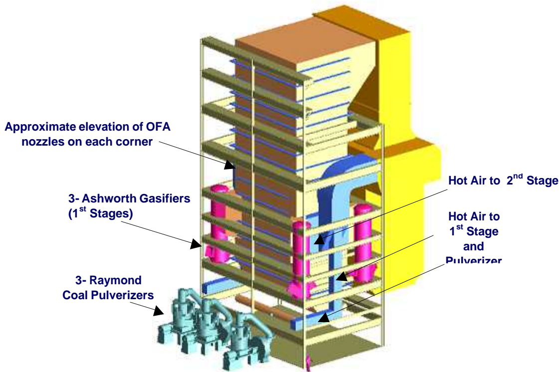
Figure 1. Three corner Ashworth gasifier firing.
