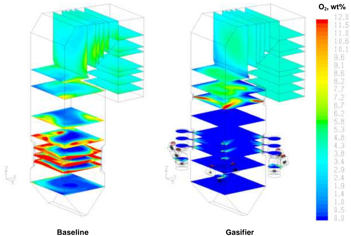
Figure 5. O 2 distribution comparison.
