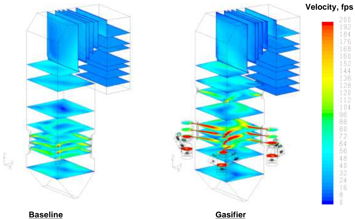
Figure 4. Horizontal plane velocities comparison.
